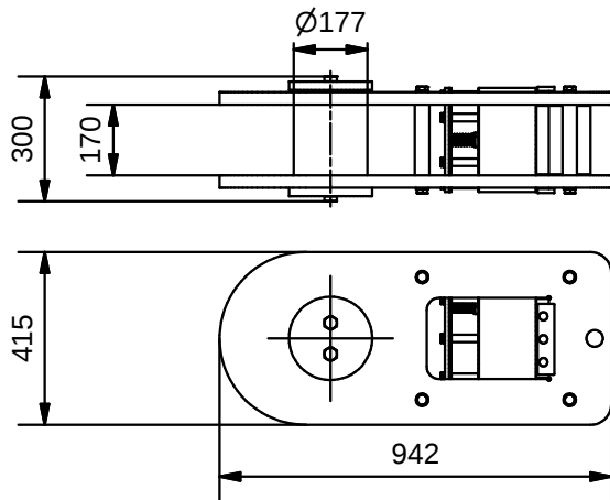
Anchor (1:20)
